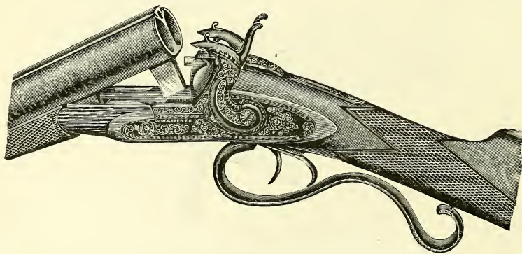
W. W. Greener's Self Half-cocking Gun, and First Top Bolt Breech-action.
